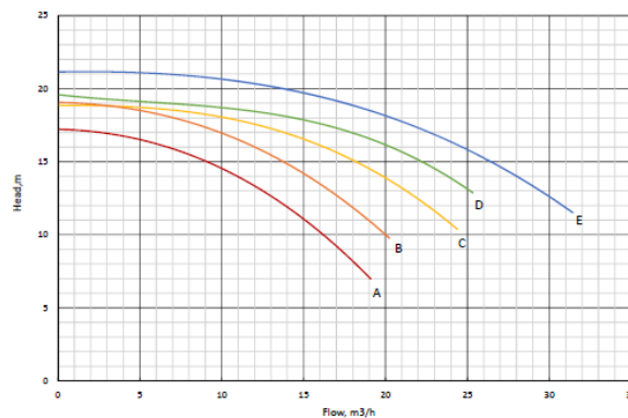
50Hz Performance Curve
